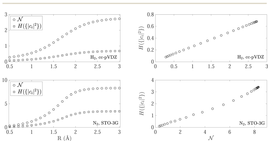
Fig. 7 Nonfreeness \mathcal{N} and Shannon entropy H(\{|c_i|_2^2\}) of the CI expansion coefficients in natural orbital basis for the full CI ground state of \text{N}_2 in the STO-3G basis at various internuclear distances R (left), and H(\{|c_i|_2^2\}) as a function of \mathcal{N} (right).
