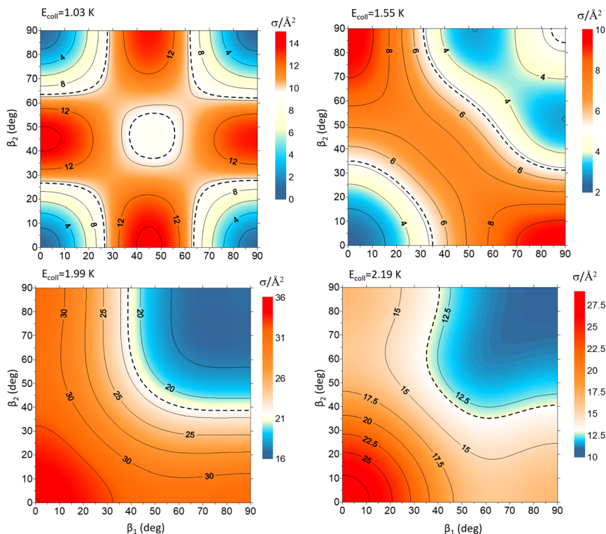
Fig. 9 Contour maps showing the \sigma^{\beta_1\beta_2} for \text{D}_2(v=2, j=2) + \text{D}_2(v=2, j=2) \rightarrow \text{D}_2(v=2, j=2) + \text{D}_2(v=2, j=0) collisions as a function of \beta_1 and \beta_2 for each of the four E_{\text{coll}} highlighted in Fig. 7. Since both \text{D}_2 molecules are indistinguishable \beta_1 and \beta_2 represent the angles that define the direction of the internuclear axis of any of the two diatoms.
