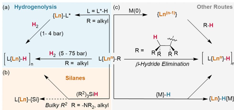
Fig. 2 Synthetic routes to lanthanide hydrides from \text{L}\{\text{Ln}\}\text{-R} complexes (a) via hydrogenolysis. \text{L}^* = metallated ligand, accessed via C–H activation/deprotonation. (b) Using silanes. (c) Other routes include reduction with alkali metals, \beta -hydride elimination and reactions with metal hydrides.
