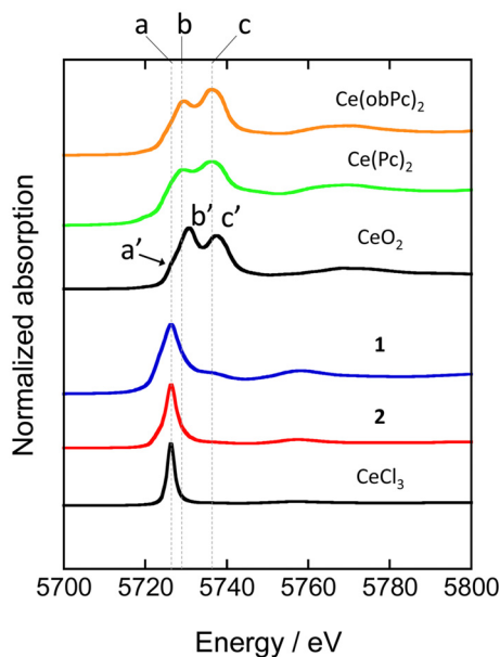
Fig. 4 Ce L III -edge XANES spectra of reference materials (CeO 2 and CeCl 3 ) and Ce(Pc) 2 based complexes. See ESI for the assignment of each peak.
