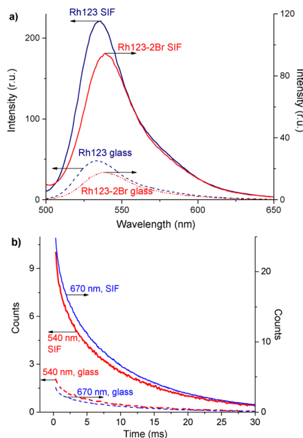
Fig. 6 (a) Fluorescence spectra of Rh123 and Rh123-2Br on the glass and SIF surfaces; (b) the time-dependence of the DF ( \lambda_{\text{reg}} = 540 \text{ nm} ) and phosphorescence ( \lambda_{\text{reg}} = 670 \text{ nm} ) decay of Rh123-2Br on the glass and SIF surfaces.
