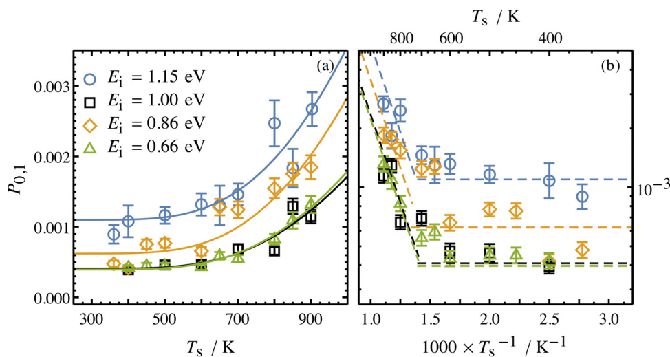
Fig. 3 Incidence energy and surface temperature dependence of HCl ( \nu = 0 \rightarrow 1 ) excitation probabilities for collisions at a Ag(111) surface shown in linear (a) and Arrhenius (b) plots. The nonadiabatic component can be discerned through its strong temperature dependence while the adiabatic component is temperature-independent. From ref. 57 with permission from American Institute of Physics Copyright (2020).
