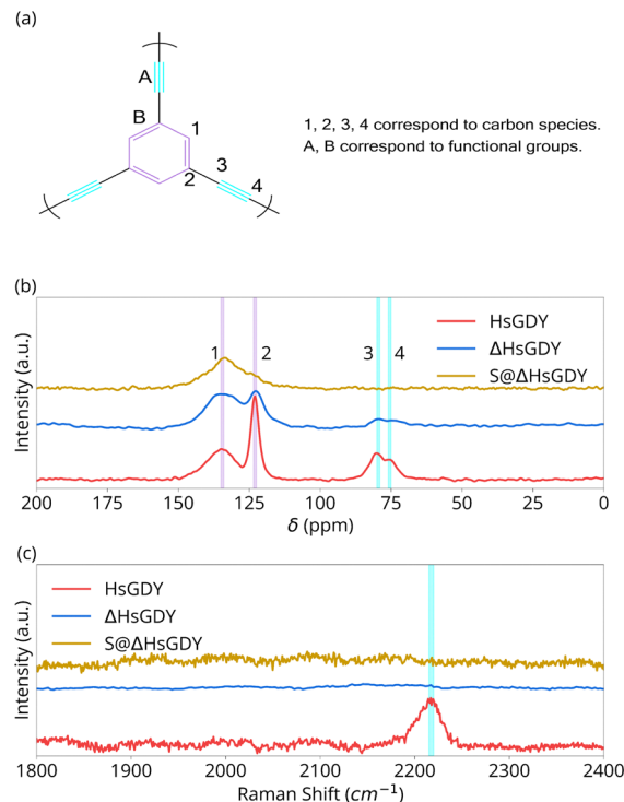
Fig. 2 Chemical characterization of HsGDY, Heated HsGDY and S@HsGDY. (a) Carbon species and functional groups in (idealized) HsGDY; (b) solid-state ^{13}\text{C} NMR; (c) Raman spectra.
