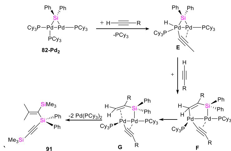
Scheme 33 Possible pathway for the formation of acyclic silane 91 from 82-Pd 2 and terminal alkynes.
