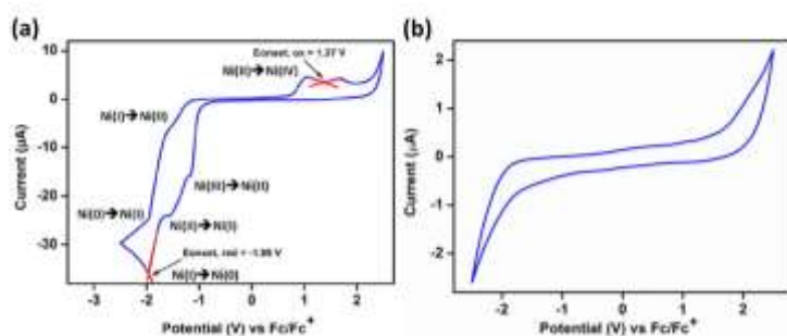
Fig. 14 CV of complex 62 in \text{CH}_2\text{Cl}_2 (a) and ligand 61 in THF (b), with 0.05 M t -butylammonium-hexafluorophosphate. All potentials were referenced to the \text{Fc}/\text{Fc}^+ couple. Scan rate = 50 \text{ mV s}^{-1} . Reproduced from Ref [35] Copyright © 2022, American Chemical Society.
