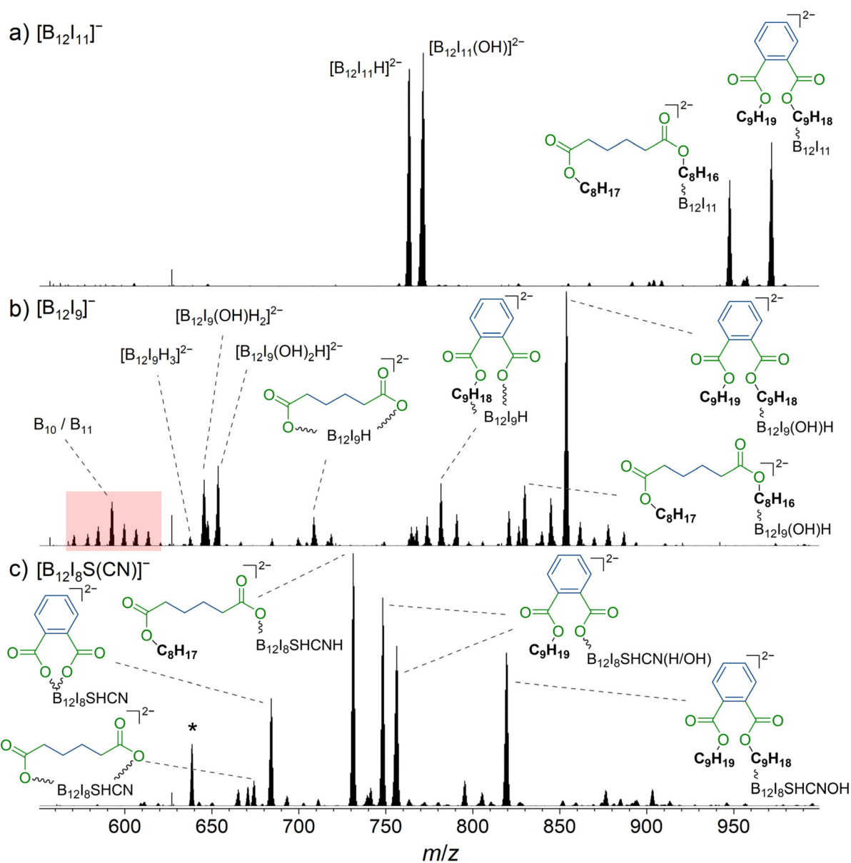
Fig. 4 Mass spectra obtained by LESA-MS after the deposition of (a) [B_{12}I_{11}]^{2-} , (b) [B_{12}I_9]^{2-} , and (c) [B_{12}I_8S(CN)]^{2-} on gold covered with FSAM. Reaction products with dinonyl phthalate and dioctyl adipate are marked with a blue organic backbone. The ester moiety is shown in green. In (b), signals assigned to fragments with m/z values smaller than that of [B_{12}I_9H_3]^{2-} are highlighted in red, indicating degradation of the B_{12} -scaffold. The isotopic pattern of the fourfold negatively charged [(B_{12}I_8(SH)(CN)H)_2(C_4H_8(COO)_2)]^{4-} is marked with an asterisk and additionally shown enlarged in Fig. 5. More detailed signal assignments are shown in Table S8.†
