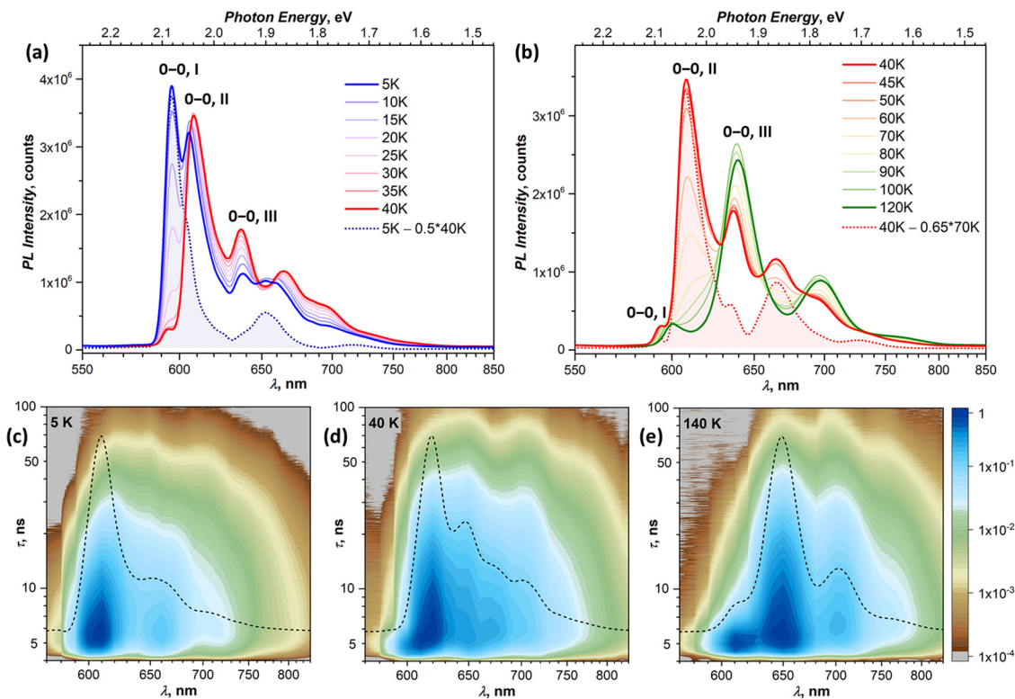
Fig. 3 (a) and (b) VT-PL spectra of DBP in the temperature ranges of 5–40 K (a) and 40–120 K (b); the blue dotted curve in (a) is the spectrum of state I obtained by a subtraction of the 40 K spectrum from the 5 K spectrum, whereas the red dotted curve in (b) is the spectrum of state II obtained as the difference of 70 K and 40 K spectra and rescaling intensity to match that at 40 K; the peaks assigned to pure electronic transitions are marked as “0–0” followed by the emissive state number. (c)–(e) ( \lambda , \tau ) maps of the PL decay at 5 K (c), 40 K (d), and 140 K (e); note that the laser pulse occurs at \tau = 4 ns and the time after the pulse is given in log scale; each map is overlaid by a quasi-CW TR spectrum (dashed curve), obtained by integration of PL decay over 100 ns after the pulse. Note that some of the features observed in the CW spectra are smeared in the TR spectra because of the lower resolution.
