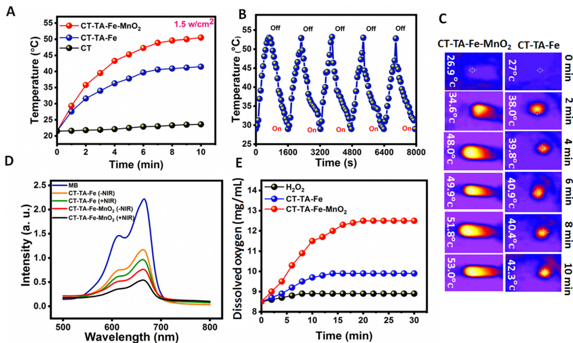
Fig. 4 (A) Photothermal properties of CT, CT-TA-Fe, and CT-TA-Fe-MnO 2 hydrogels (500 \mu\text{g mL}^{-1} ) under 808 nm laser irradiation with a power density of 1.5 \text{W cm}^{-2} . (B) Temperature vs. time curve for CT-TA-Fe-MnO 2 (500 \mu\text{g mL}^{-1} ) irradiated with an 808 nm laser (1.5 \text{W cm}^{-2} ) for five on-off cycles (on: 10 min; off: 10 min). (C) NIR thermal images of CT-TA-Fe and CT-TA-Fe-MnO 2 under 808 nm laser irradiation at different times. (D) UV-vis spectrum of MB after different treatments with CT-TA-Fe and CT-TA-Fe-MnO 2 hydrogels with/without NIR light. (E) Oxygen release by CT-TA-Fe and CT-TA-Fe-MnO 2 hydrogels in the presence of H 2 O 2 measured by a commercial oxygen meter.
