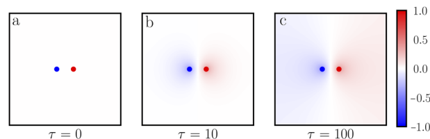
Fig. 8 Concentration field generated by a point source and sink dipole. (a–c) \tilde{c}(\vec{r}, \tau) at \tau = 0, 10, 100 for a dipole with d = 3 and a molar rate \mathcal{J}(\tau) = \mathcal{H}(\tau) . The color bar ranges between -1 and 1 and represents the value of \tilde{c}(\vec{r}, \tau) . The point source and sink are visualized as a red and blue circle and are not representative of solute concentration at the location of the source and sink.
