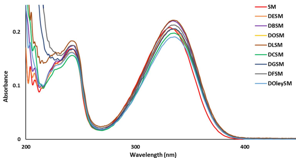
Fig. 2 UV spectra of SM and SM diesters in EtOH.
