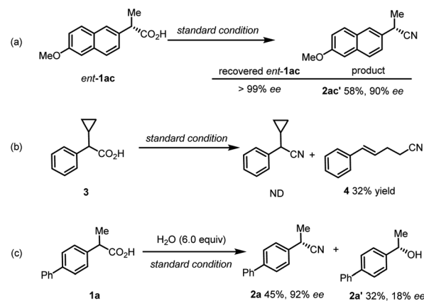
Scheme 3 Mechanistic studies.
