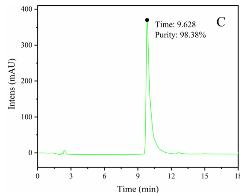
Fig. 3 HPLC spectra of W1 (myricetin-3-O-glucoside) (A), W2 (myricetin-3-O-arabinoside) (B), and W3 (myricitrin) (C).
