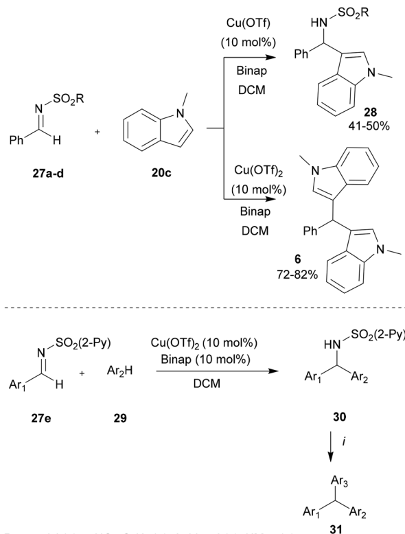
Scheme 7 One-pot synthesis of unsymmetrical triarylmethanes through a copper-catalyzed aza-FC reaction. R = p -tolyl ( a ), p - \text{NO}_2 - \text{C}_6\text{H}_4 ( b ), 2-thienyl ( c ), \text{NMe}_2 ( d ) \text{Ar}_1, \text{Ar}_2, \text{Ar}_3 = indolyl, (5-OMe)- N -methylindolyl, 2,4,6-triOMePh, 2-OMe-thiophenyl... i : if \text{Ar}_2 = indolyl: \text{Ar}_3\text{H} , 40°C (one-pot); for other aromatic groups: \text{Ar}_3\text{H} , \text{Sc}(\text{OTf})_3 10 mol%, ACN, 60°C
