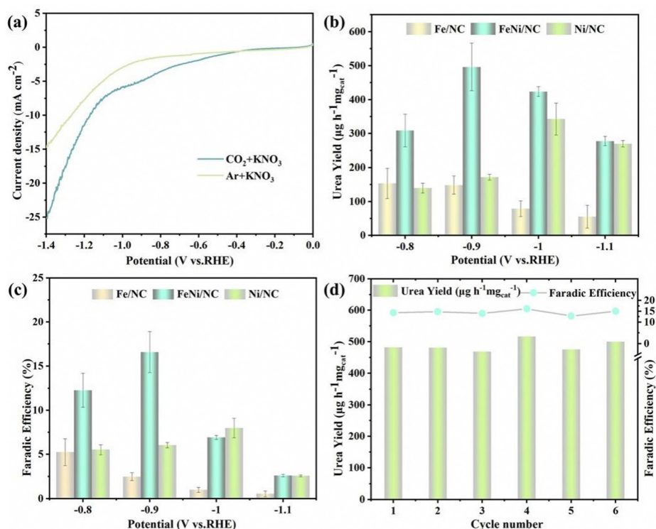
Fig. 3 (a) LSV curves of FeNi/NC measured in Ar and \text{CO}_2 saturated 0.1 \text{ M KNO}_3 electrolytes. (b) The urea yield and (c) urea FE for FeNi/NC, Fe/NC, and Ni/NC on the different applied potentials. (d) The cyclic stability test of FeNi/NC for urea synthesis.
