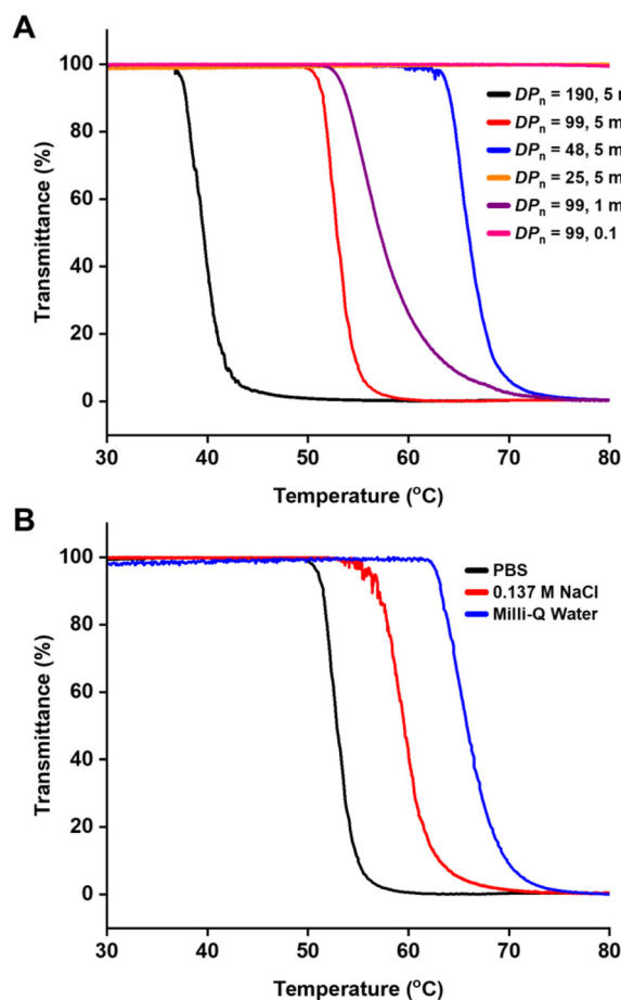
Fig. 4 Turbidity measurements of (A) PBS solutions of P(MAmBA) of different DP n and concentrations; and (B) P(MAmBA) 99 solutions in different media (5 mg ml -1 ).
