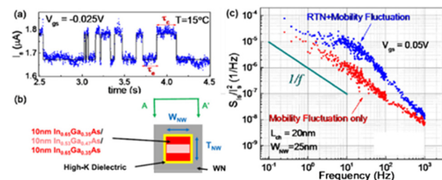
Fig. 20 (a) RTN at V_{\text{DS}} = 50 \text{ mV} for InGaAs NW MOSFET with geometry illustrated schematically in (b). The gate dielectric of the device in (a) is 0.5 nm \text{Al}_2\text{O}_3/4.0 \text{ nm} \text{LaAlO}_3 . (c) Normalized noise power spectral density vs. frequency for two InGaAs NW MOSFETs with 3.5 nm \text{Al}_2\text{O}_3 dielectrics: one showing RTN and the other showing LF noise. Adapted from ref. 67 with permission. Copyright 2015 Institute of Electrical and Electronics Engineers.
