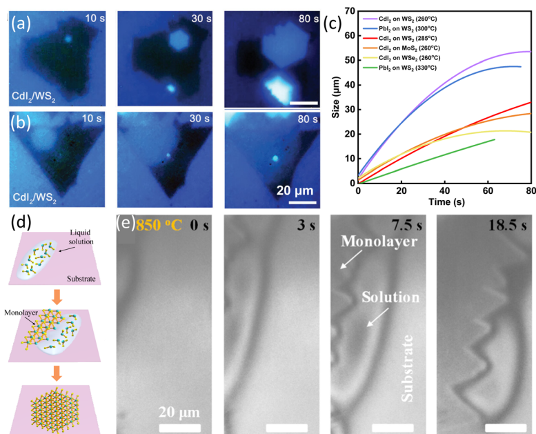
Fig. 3 Schematic illustration of in situ imaging the growth rate of M 12 (M = Cd, Pb) and MoS 2 . (a) In situ real-time images of the growth process of Cd 12 /WS 2 heterostructure at a growth temperature of 285 °C. (b) In situ real-time images of the growth process of Cd 12 /WS 2 heterostructure at a growth temperature of 260 °C. (c) Plotting of the size of M 12 (M = Cd, Pb) with time at different temperatures. Reproduced from ref. 76 with permission from Wiley, copyright 2021. (d) Illustration of the LPEE process of TMDs. (e) In situ imaging of LPEE of MoS 2 monolayers from the CsCl solution at 850 °C. Reproduced from ref. 78 with permission from American Chemical Society, copyright 2023.
