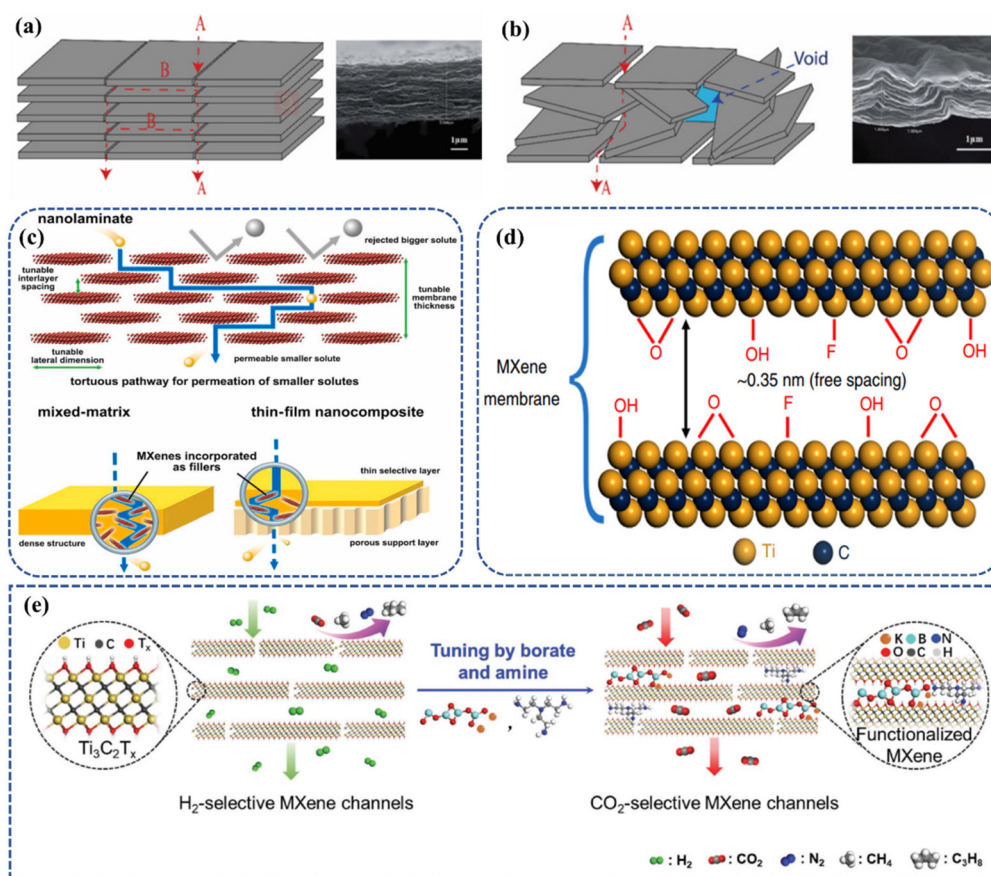
Fig. 14 Schematic diagrams of two mass transport mechanisms (a) through in-plane fissure-like pores (A) and interlayer channels (B). (b) Voids formed between the less ordered MXene nanosheets. Reprinted with permission. 176 Copyright 2022, the American Chemical Society. (c) Separation mechanism of MXene-based membrane. Reprinted with permission. 77 Copyright 2020, John Wiley and Sons. (d) Schematic diagram of adjacent MXene nanosheets. Reprinted with permission. 75 Copyright 2018, Springer Nature. (e) Schematic diagram of the selective permeation of H 2 and CO 2 in MXene membrane. Reprinted with permission. 73 Copyright 2018, John Wiley and Sons.
