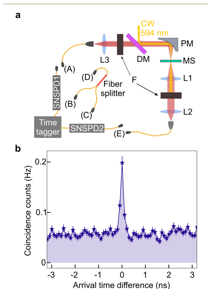
Fig. 2 (a) The experimental setup. The pump, a CW laser at 594 nm, is fed through dichroic mirror DM and focused on the metasurface (MS) with parabolic mirror PM. The same PM collimates backward emitted photons, while forward emitted photons are collimated by lens L1. After the pump is removed with bandpass and long-pass filters F, lenses L2, 3 couple SPDC photons into single-mode fibers connected to two superconducting-nanowire single-photon detectors (SNSPD 1, 2). Depending on what configuration of SPDC (forward, backward, or bi-directional) is studied, SNSPDs are connected, respectively, either both, through a fiber beamsplitter, to output port E, or both to output port A, or one detector to output E and the other, to output port A. (b) The coincidence histogram for bidirectionally emitted photons from a 70 mW pump.
