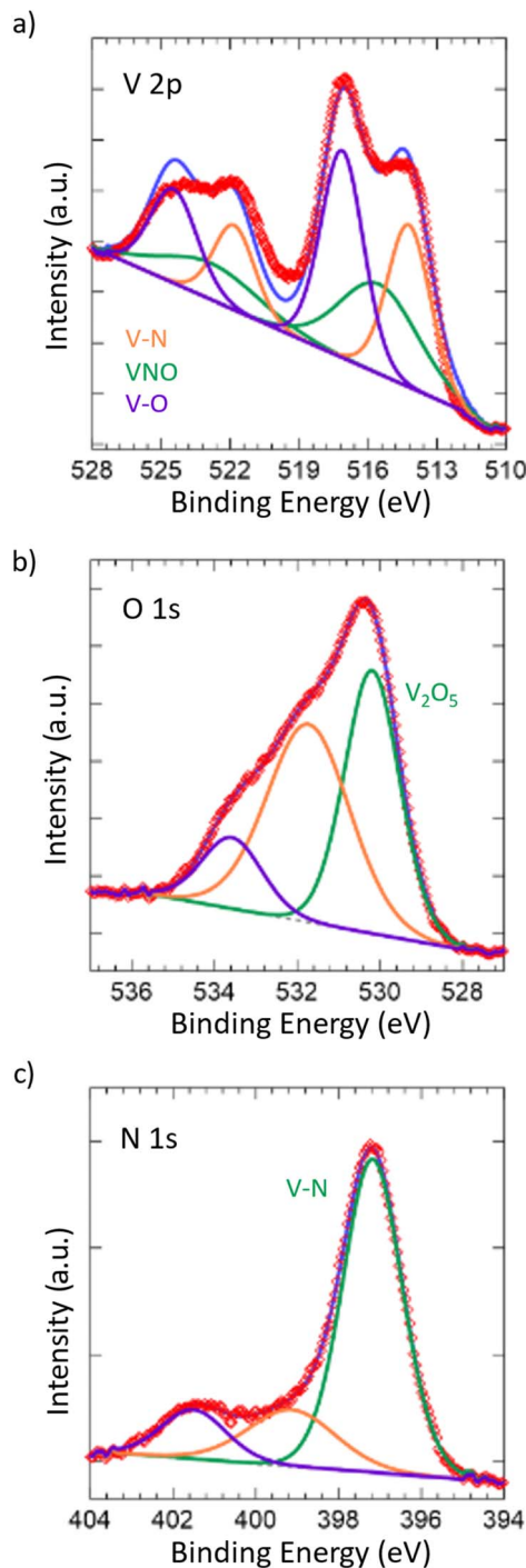
Fig. 2 XPS spectra of (a) V 2p, (b) O 1s, and (c) N 1s for the synthesized VN. All spectra are plotted with respect to reference values. The degree of surface oxidation and amount of pristine vanadium nitride structure were tracked according to the V 2p, O 1s, and N 1s spectra.
