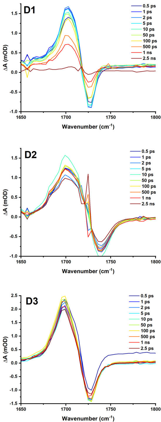
Fig. 8 TRIR spectra of D1, D2 and D3 in DCM following excitation at 525, 500 and 500 nm respectively (2 mW, OD@_{\lambda_{ex}} \sim 0.6 ), collected with the pump set to magic angle ( 54.7^\circ ) with respect to the probe. The time delay between the pump and probe for each spectrum is shown in the legend. Kinetic traces are shown in the ESI.†
