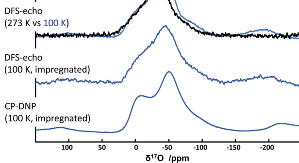
Fig. 4 ^{17}\text{O} MAS NMR spectra of (a) m -CPPT \beta and (b) t -CPPD after ^{17}\text{O} -labelling using BM, recorded at different magnetic fields (9.4, 14.1, 18.8 and 35.2 T). Zoom into the lineshapes recorded at 35.2 T is provided in the ESI (Fig. S3†). (c) Low-temperature ^{17}\text{O} MAS NMR and DNP-enhanced NMR analyses of the m -CPPT \beta phase at 14.1 T (see experimental section for details). “*” symbols correspond to spinning sidebands.
