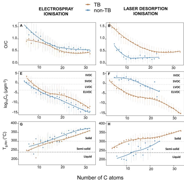
Fig. 5 Average values of O/C, \log_{10} of estimated saturation mass concentration ( \log_{10}C_0 ), and relative-humidity dependent glass transition temperature ( T_{g, \text{RH}} ) against the number of C atoms in the formulae assigned. Components exclusively identified in BBAug1318 (TB-rich) are plotted relative to non-TB components (identified in BBAug1011, BBAug0910 (NT), and/or BBAug09 (DT)). In (–)ESI, all three non-TB aerosol samples were considered, while for (–)LDI, non-TB refers to BBAug0910 (NT) and BBAug1011 only.
