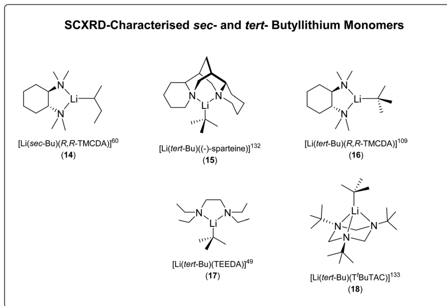
Fig. 15 The SCXRD-characterised s BuLi ( 14 ) and t BuLi ( 15–18 ) monomers.
