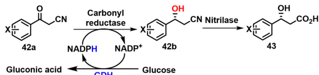
Scheme 21 The biosynthesis route to (R)-β-hydroxy carboxylic acids.
