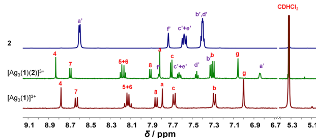
Fig. 1 Partial 1 H NMR (600 MHz, CD 2 Cl 2 , 298 K) of silver(i)-loaded deck [Ag 3 ( 1 )( 2 ) 3 ] 3+ , slider-on-deck [Ag 3 ( 1 )( 2 ) 3 ] 3+ and biped 2 .
