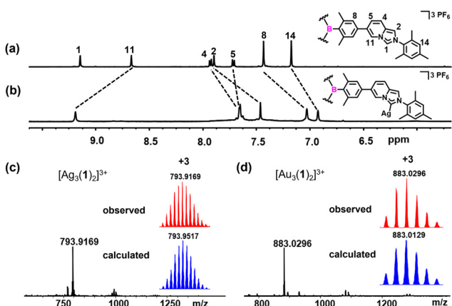
Fig. 1 Sections of the ^1H NMR spectra (600 MHz, CD_3CN ) of (a) H_3-1(PF_6)_3 and (b) [Ag_3(1)_2](PF_6)_3 . The HR-ESI mass spectra of (c) [Ag_3(1)_2]^{3+} and (d) [Au_3(1)_2]^{3+} (experimental in red, calculated in blue).
