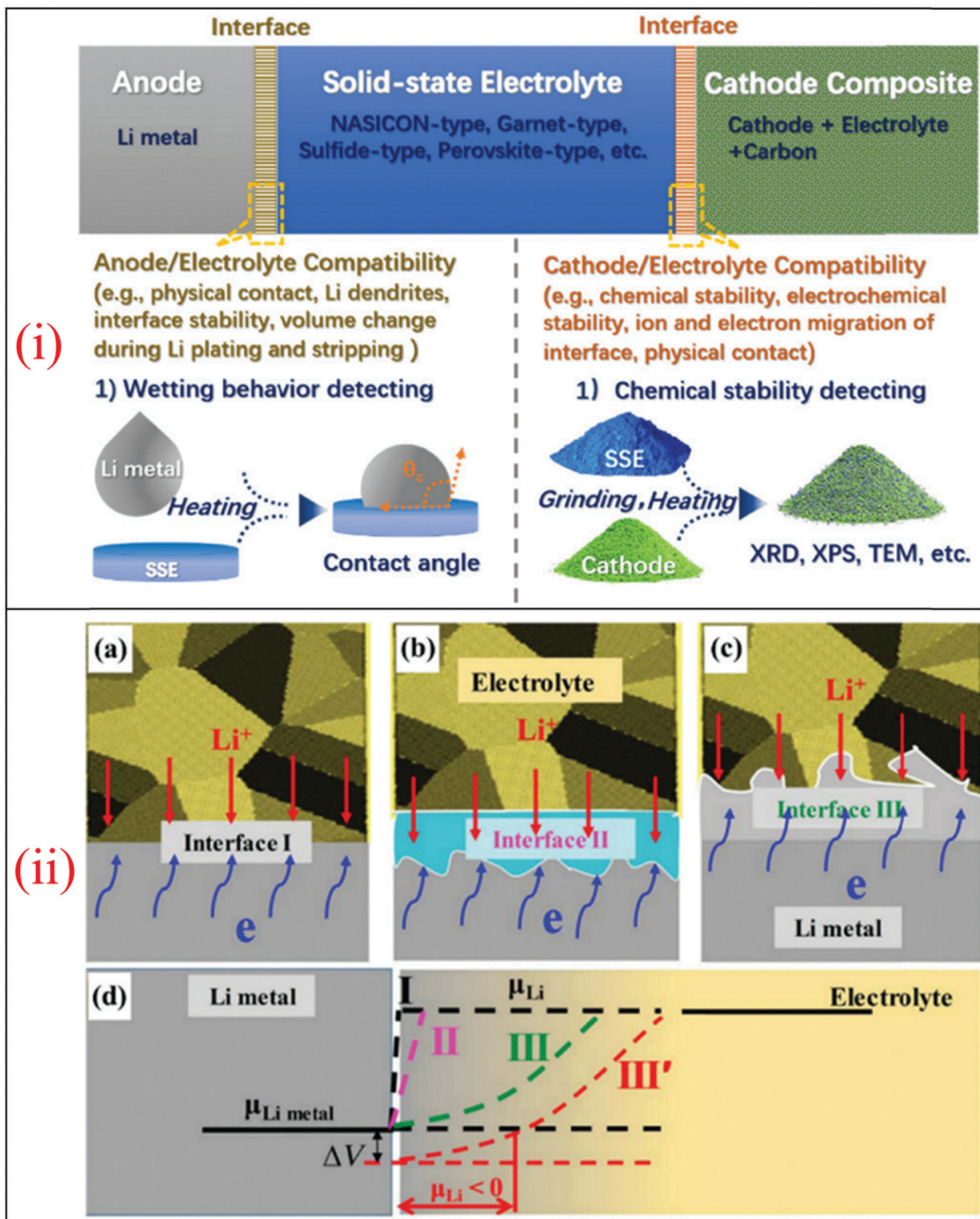
Fig. 16 (i) Summary of compatibility problems associated with interfaces in SSBs (Fig. 1 from ref. 322). (ii) Formation of different types of Li/SSE interphases. (a) Intrinsic stable interface between the Li metal and the SSE. (b) Metastable solid-electrolyte interphase between the Li metal and the SSE. (c) Reactive mixed-conducting interphase between the Li metal and the SSE. (d) Corresponding Li potentials between the Li metal and different SSEs. 322
