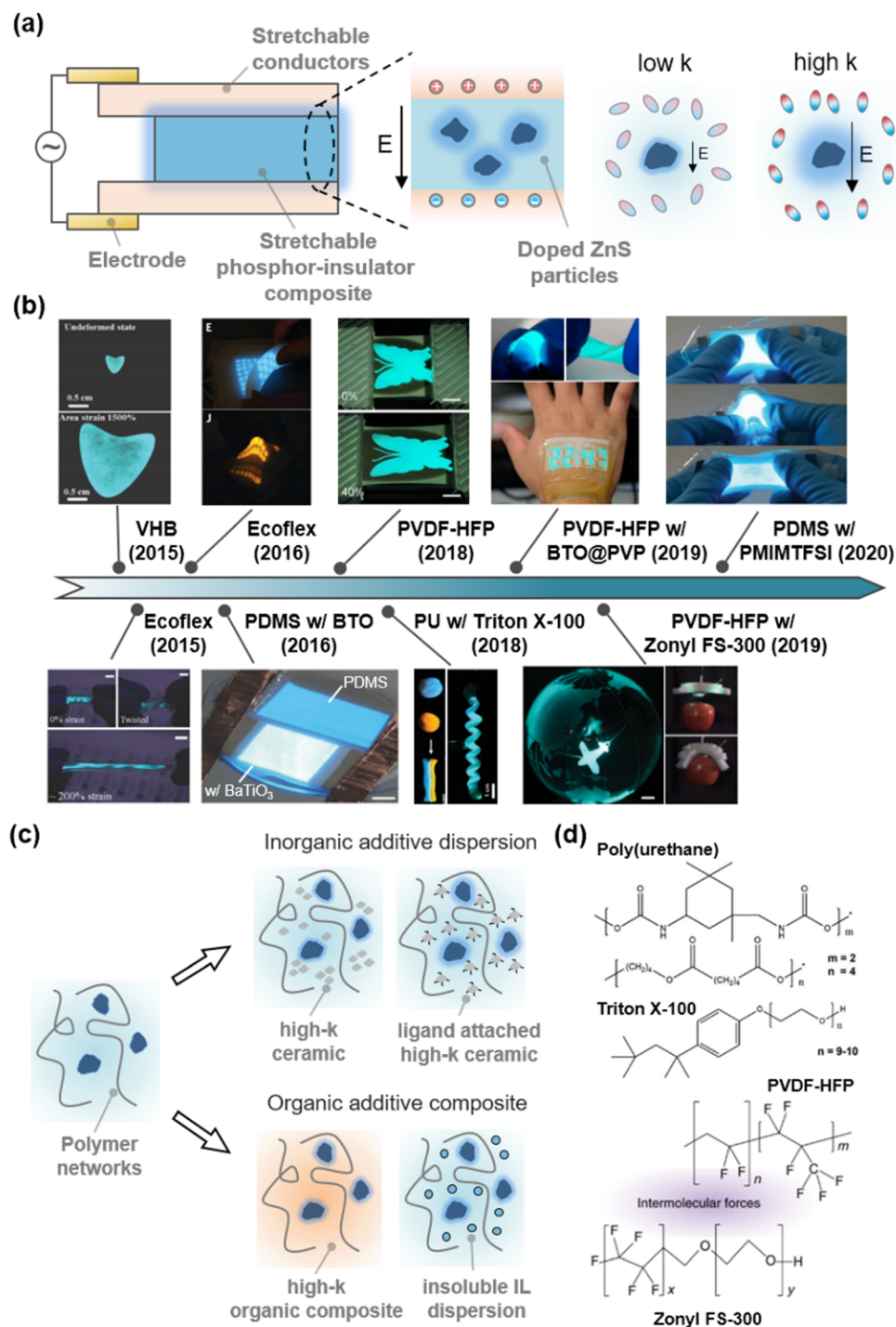
Fig. 16 High- k SIs for low-voltage optoelectronics. (a) Structure of stretchable alternate-current-electroluminescence (AC-EL) devices. The phosphors exhibit higher luminescence under an electric field, when the surrounding medium has higher dielectric constants. (b) Materials development for low voltage stretchable AC-EL devices. Reproduced with permission from ref. 155, 156, 157, 158 and 159. Copyright 2015, 2016, 2018, and 2020, Wiley-VCH. Reproduced with permission from ref. 26. Copyright 2016, AAAS. Reproduced with permission from ref. 160 and 161. Copyright 2018, and 2019, The American Chemical Society. (c) Schematics of strategies used to develop high- k stretchable dielectrics. (d) Molecular structures comprising high- k organic composites. Reproduced with permission from ref. 162. Copyright 2019, Springer Nature.
