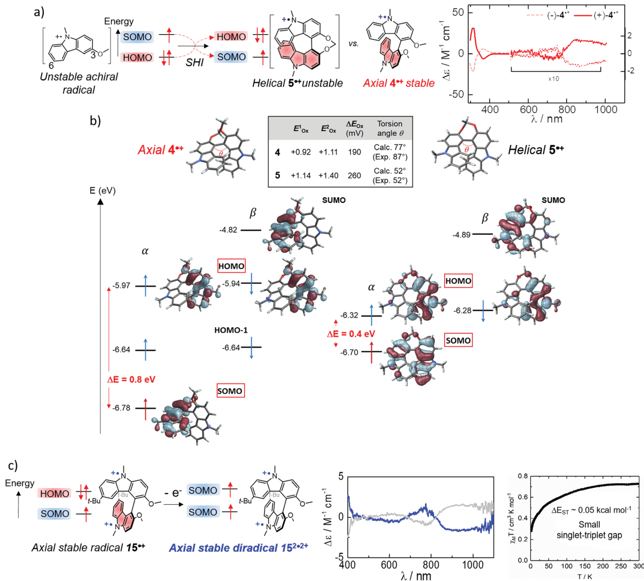
Fig. 13 (a) Axially and helically chiral SHI cationic bicarbazole monoradicals 4^{++} and 5^{++} , and orbital comparison with their common non-SHI cationic carbazole radical precursor, with the near IR circular dichroism of (+) and (–)- 4^{++} (counter anions are omitted for clarity); (b) calculated orbital energies (in eV) and isosurfaces ( \pm 0.030 ) of frontier molecular orbitals computed for monoradicals 4^{++} (left) and 5^{++} (right). The HOMO–SOMO energy differences are averaged over the highest occupied spin orbital energies. Oxidation potentials and separation of the two first oxidation potentials in V vs. SCE, theoretical (calc.) and experimental (exp.) dihedral angles between the carbazole fragments; (c) schematic illustration of the electronic configuration of diradical 15^{2+2+} obtained upon oxidation of SHI radical 15^{++} , near IR circular dichroism of (+) and (–)- 15^{2+2+} in acetonitrile at 298 K, and its magnetic susceptibility ( \chi_M T vs. T ). Figures adapted with permission from ref. 74. Copyright 2020 American Chemical Society.
