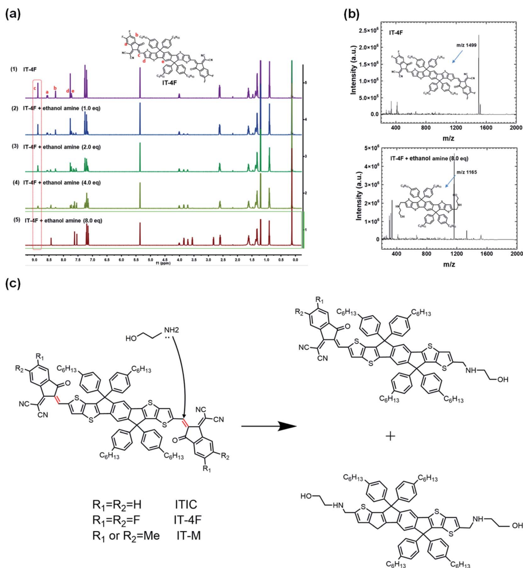
Fig. 4 (a) In situ 1 H NMR spectra of pristine IT-4F and IT-4F after adding different equivalents of ethanolamine; (b) the mass spectra of pristine IT-4F and IT-4F after adding 8.0 eq. ethanol amine, respectively. The detection was operated in negative ion mode; (c) reaction scheme of NFA of ITIC and ethanolamine. Reproduced from ref. 43 with permission from the Nature Publishing Group, copyright [2020].
