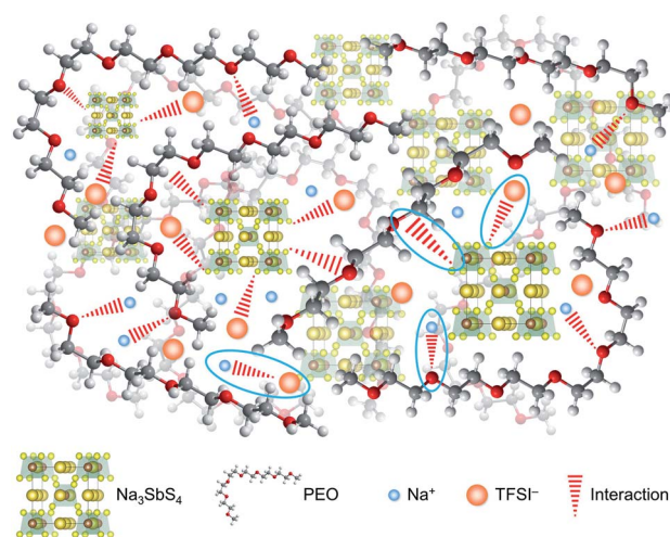
Fig. 4 Schematic diagram of the structure of the PEO/NaTFSI/ Na_3SbS_4 electrolyte, where the four types of interactions between the different components ( Na_3SbS_4 and TFSI − , Na_3SbS_4 and PEO, Na^+ and PEO, Na^+ and TFSI − ) are highlighted.
