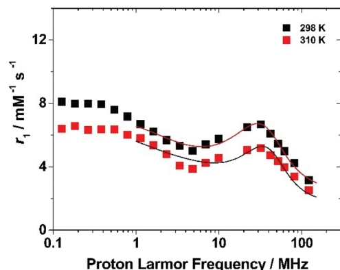
Fig. 6 Nuclear magnetic relaxation dispersion (NMRD) profiles of Gd-L 1 -P particles (0.89 mM) at 298 (black squares) and 310 K (red squares). The solid lines represent the best results of the fitting to the experimental points.
