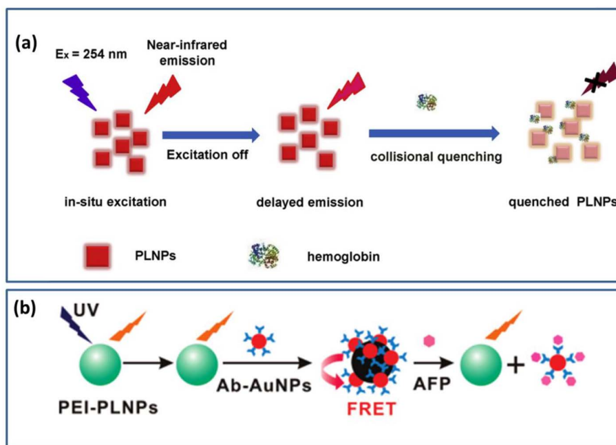
Fig. 6 (a) Schematic diagram for ultra-sensitive detection of hemoglobin. Reproduced from ref. 82 with permission from Elsevier, copyright 2020. (b) Schematic diagram of these PLNPs for the determination of AFP content. Reproduced from ref. 168 with permission from the American Chemical Society, copyright 2011.
