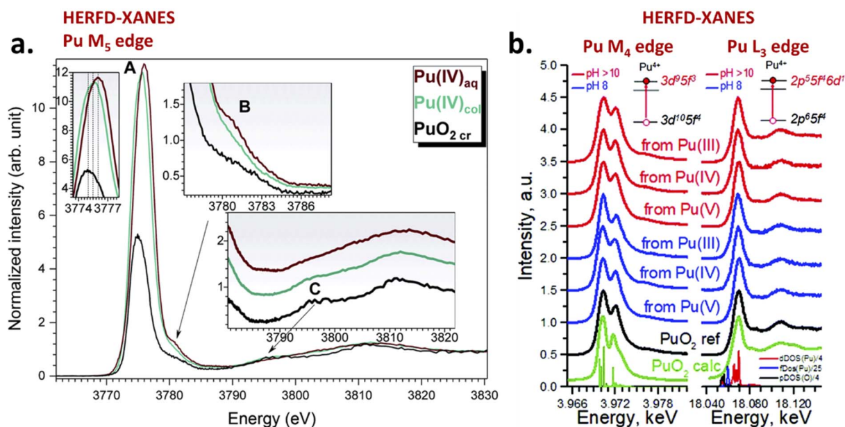
Fig. 19 (a) HERFD-XANES spectra acquired at the Pu M 5 edge for aqueous Pu(IV) containing 6% Pu(V), bulk PuO 2 and Pu(IV) colloids. Adapted from Vitova et al. 124 with permission from the Royal Society of Chemistry, copyright 2018. (b) HERFD-XANES spectra acquired at the Pu M 4 edge for PuO 2 nanoparticles prepared by the addition of ammonia to Pu(III–V) aqueous solutions. Adapted from Gerber et al. 111 with permission from the Royal Society of Chemistry, copyright 2020.
