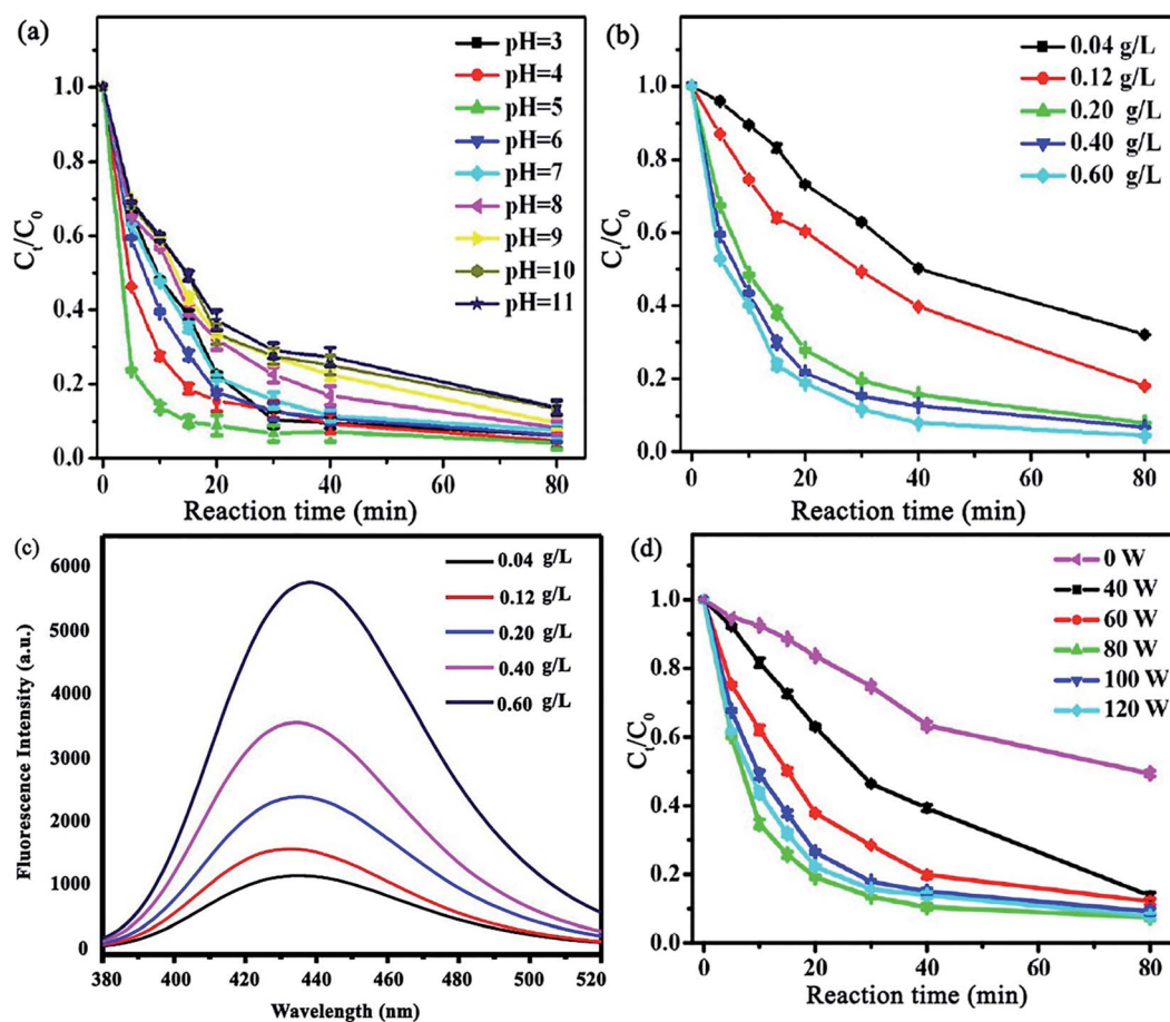
Fig. 20 Effect of various parameters on TC removal: (a) solution pH, (b) Fe/N-C-2 concentration, and (c) influence of Fe/N-C-2 concentration ( g L^{-1} ) on \cdot OH production utilizing a terephthalic acid fluorescence probe. (Reaction conditions: 60 mM terephthalic acid concentration; 60 mM H_2O_2 ; reaction temperature: 25 °C; 80 W US power; and 80 min reaction time). (d) Ultrasonic power. This figure was adapted with permission from: ACS Omega , 2018, 3, 15870–15878. 136
