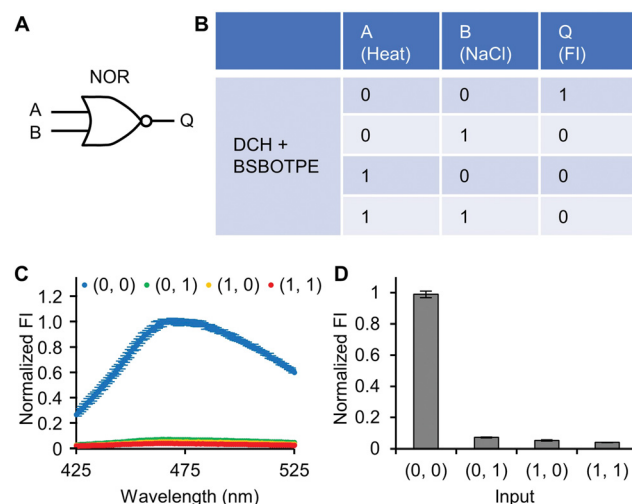
Fig. 7 NOR logic operation. (A) Symbol of logic gate. (B) Truth table. (C) The normalized fluorescence spectra of logic operation with different inputs. (D) Normalized FI at 471 nm. The concentrations of DCH and BSBOTPE used are 6 \mu\text{M} and 141 \mu\text{M} , respectively. Excitation wavelength was set at 350 nm. The 'heat' input is incubation under 40 ^{\circ}\text{C} for 2 min. The 'NaCl' input is increasing NaCl concentration from 150 mM to 600 mM, followed by 2-min incubation. n = 3 .
