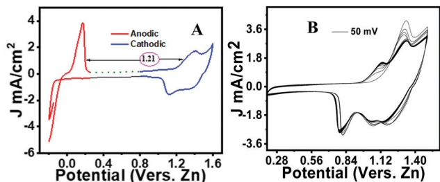
Fig. 2 (A) Cyclic voltammograms of zinc and neat phenothiazine showing the output cell voltage of 1.21 V. (B) Multiple voltammograms showing the poor stability during multiple scans (cyclic voltammograms of the neat phenothiazine-coated glassy carbon electrode as the working and zinc plate as the counter and reference electrodes in 2 M ZnSO 4 ).
