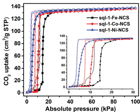
Fig. 2 \text{CO}_2 sorption isotherms for sql-1-M-NCS ( M = \text{Fe} , \text{Co} , and \text{Ni} ) at 195 K. The solid and open symbols represent adsorption and desorption branches, respectively.
