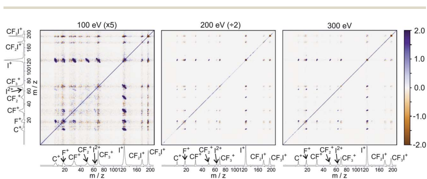
Fig. 5 ToF–ToF covariance maps obtained following electron ionisation of \text{CF}_3\text{I} at electron energies of 100, 200, and 300 eV. Saturated ToF–ToF covariance maps for the 200 and 300 eV data, in which weaker covariance signals are visible, can be found in the ESI.†
