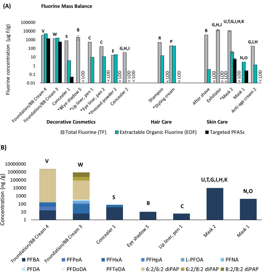
Fig. 3 (a) Fluorine mass balance showing TF, EOF and targeted PFAS concentrations ( \mu\text{g F g}^{-1} sample). The targeted PFAS ( \Sigma\text{PFAS} ) concentrations were converted to fluorine concentrations for comparative purposes. ( \text{LOD}_{\text{TF}} = 35.45 \mu\text{g F g}^{-1} , \text{LOD}_{\text{EOF}} = 0.32 \mu\text{g F g}^{-1} , \text{LOD}_{\Sigma\text{PFAS}} = 0.0015 \mu\text{g F g}^{-1} ). *Mica listed among ingredients; #synthetic fluorophlogopite listed among ingredients. (b) Concentrations ( \text{ng g}^{-1} sample) of targeted PFAS in 5 decorative cosmetics and 2 skin care samples (masks). Samples not shown (8 out of 15) were <\text{LOD} . Samples are plotted on a logarithmic scale (base 10) to enhance readability. The letters on top of each bar correspond to structures provided in Fig. 2.
