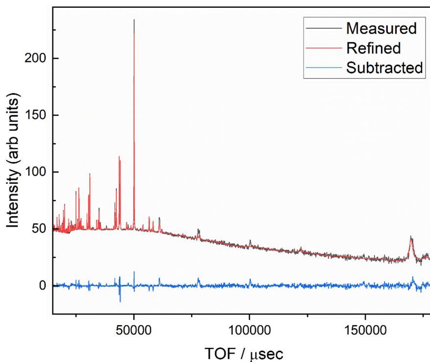
Fig. 1 PND diffractogram of BGC with Rietveld refinement to orthorhombic Pmmm .
