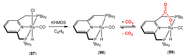
Scheme 31 The first example of the use of dearomatization MLC for the activation of CO 2 .
