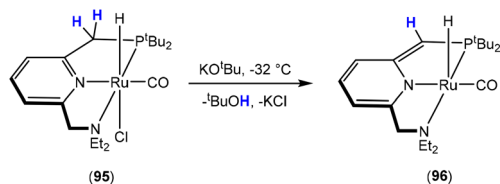
Scheme 29 Initial discovery of dearomatization by Milstein and co-workers; proton is removed from the ligand rather than the metal centre.
