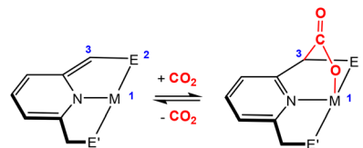
Scheme 30 Generalised scheme highlighting the potential for reversible CO 2 activation via MLC involving dearomatization–aromatization. This is a 1,3-addition across a two-atom bridge.
