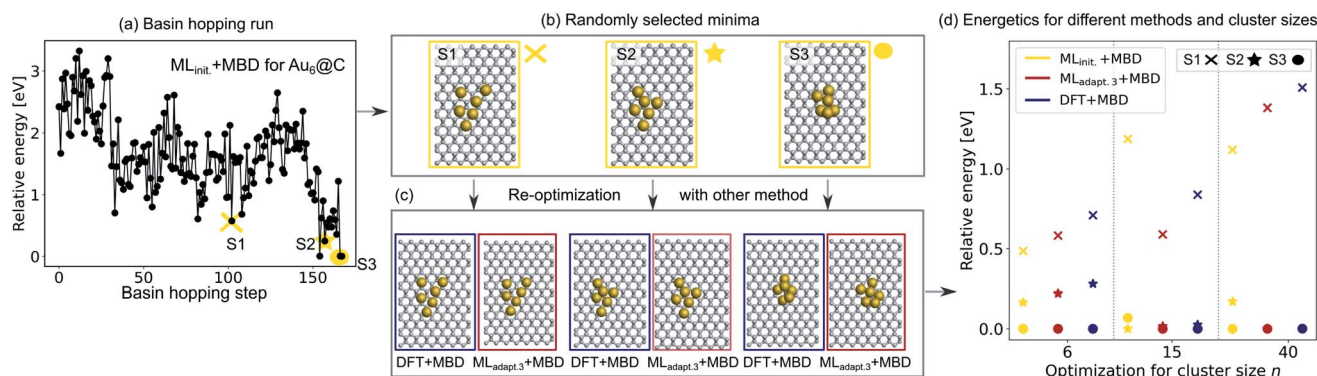
Fig. 4 (a) Basin hopping run with ML_{\text{init}} for Au@C with Au 6 nanoclusters (NCs). Yellow circles indicate (b) 3 selected structures S1–S3 that include the energetically lowest geometry and two randomly selected structures according to ML_{\text{init}} , that are (c) reoptimized with DFT+MBD (blue) and ML_{\text{adapt.3}} +MBD (red). (d) Relative energies reported with respect to the energetically lowest cluster for each method. In addition, energy rankings of the energetically lowest structures and two randomly selected structures from basin hopping runs with NC sizes of 15 and 40 atoms using ML_{\text{init}} +MBD (yellow), ML_{\text{adapt.3}} +MBD (red), and DFT+MBD (blue). Corresponding structures are shown for each method in Fig. S2.†
