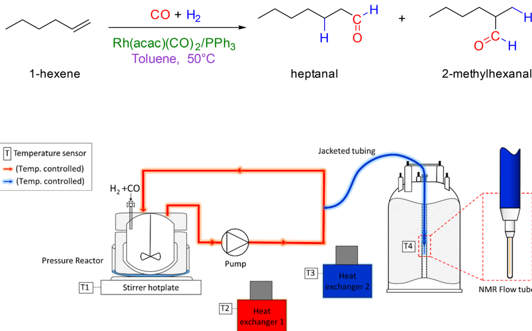
Fig. 4 Reaction conditions of the hydroformylation of 1-hexene (upper) and schematic of the FlowNMR apparatus (lower).
