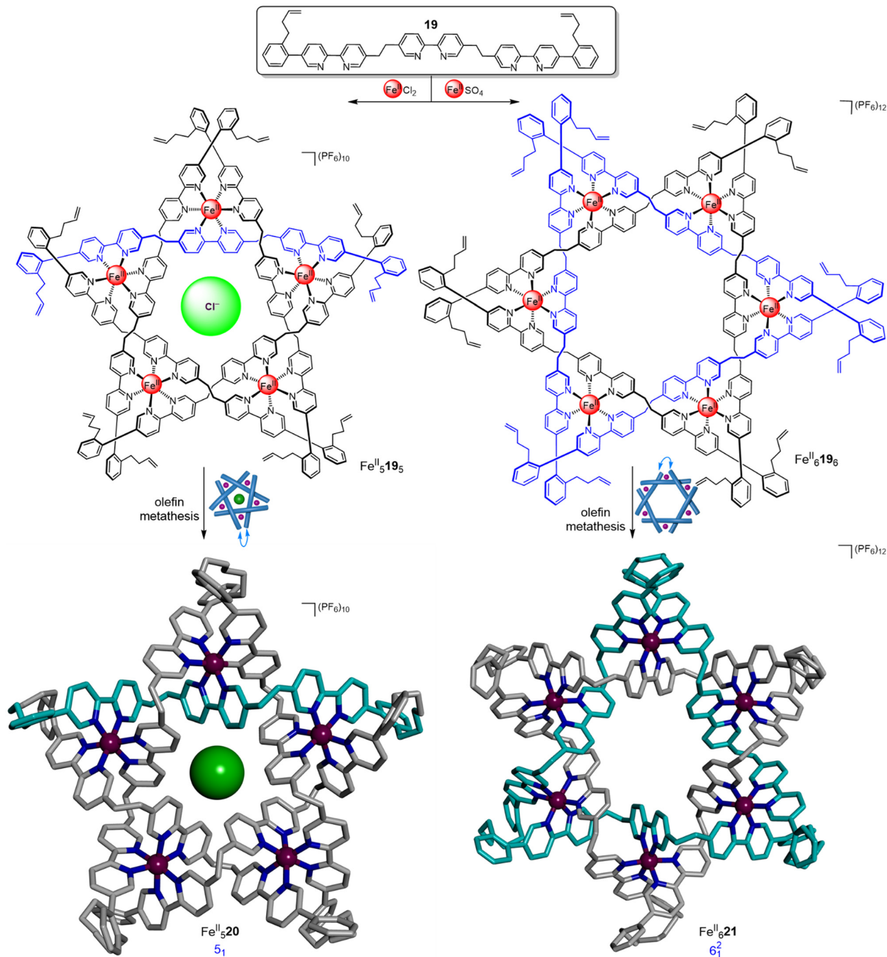
Fig. 7 Generation of hexameric and pentameric circular helicates and their subsequent closure by olefin metathesis to form a pentafoil knot \text{Fe}^{\text{II}}_{20} 55 and a Star of David triply interlocked [2]catenane \text{Fe}^{\text{II}}_{21} . 56
