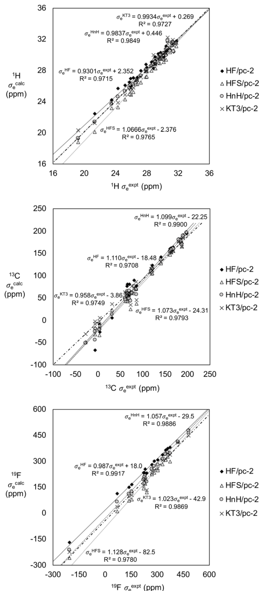
Fig. 1 Computed vs. semi-experimental equilibrium shieldings for ^1\text{H} (top), ^{13}\text{C} (middle) and ^{19}\text{F} (bottom) nuclei.
